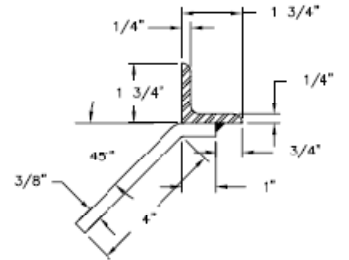
SECTION DETAIL
