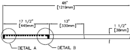
GRATE SECTION
